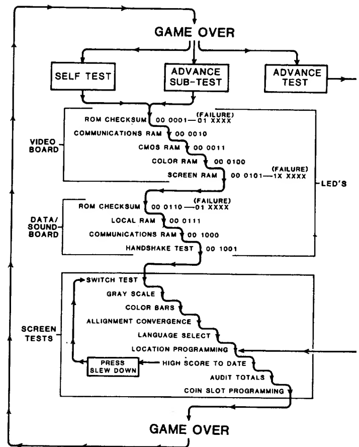
FIGURE 1-8 FLOW CHART
