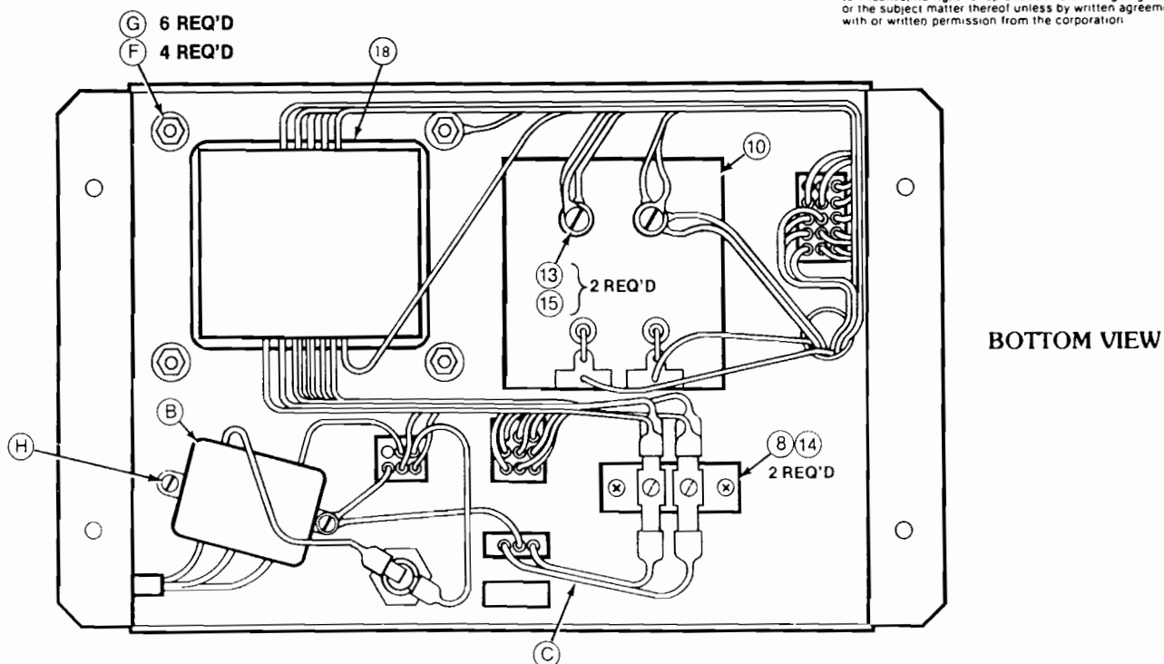
Figure 18 Power Supply Assembly for X-Y Games A034561-02 D
