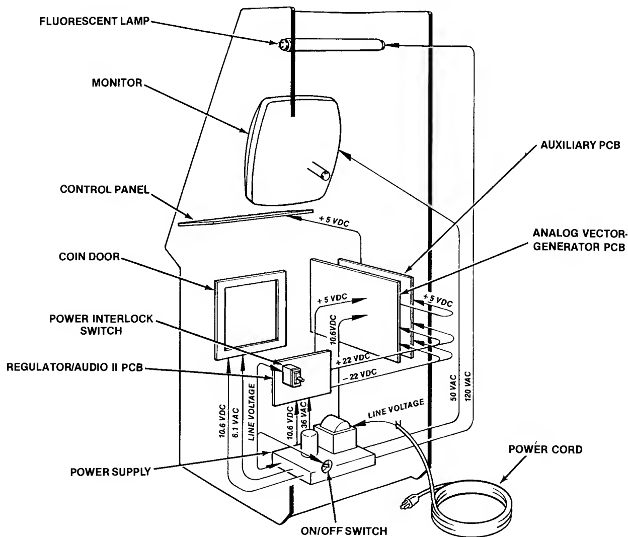
Figure 16 Power Distribution
