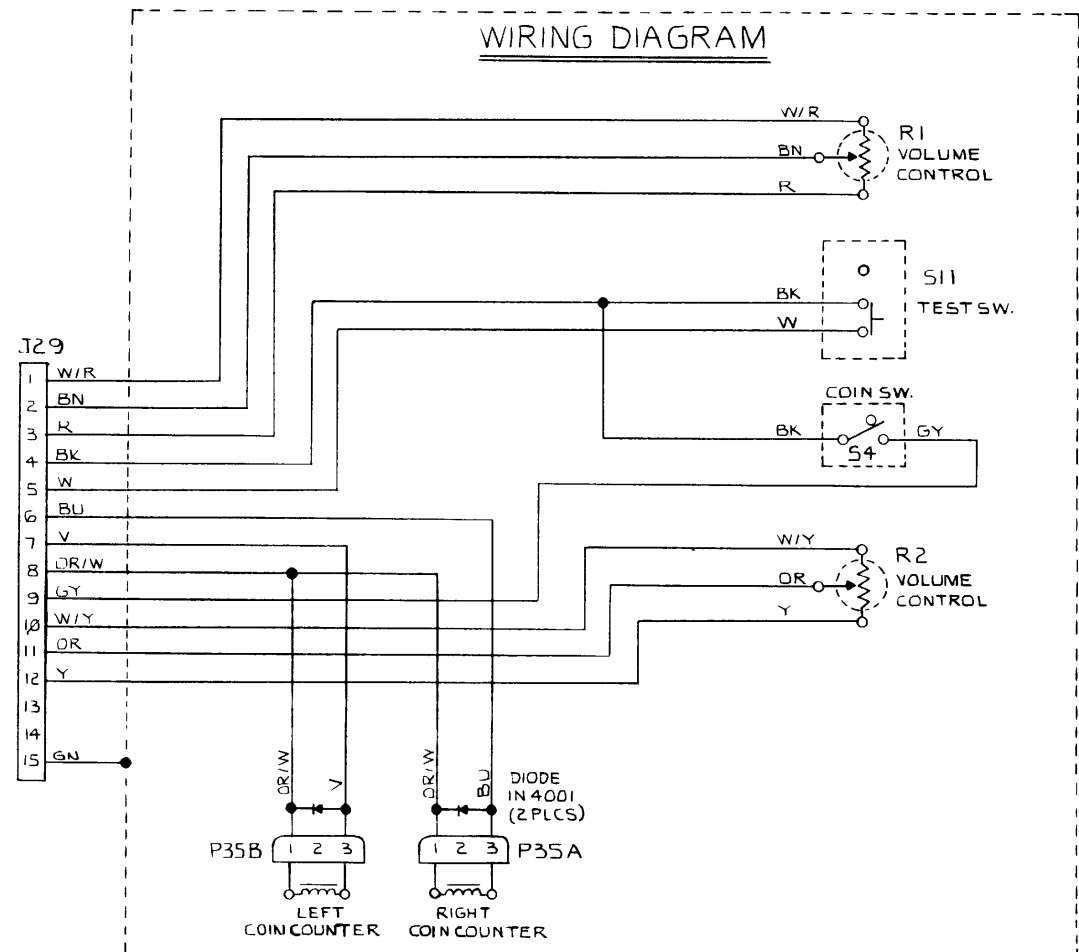
Utility Panel Wiring Diagram
