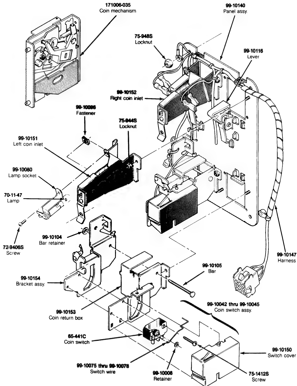
Figure 5-7 American-Made Coin-Door Assembly 171027-001 A
