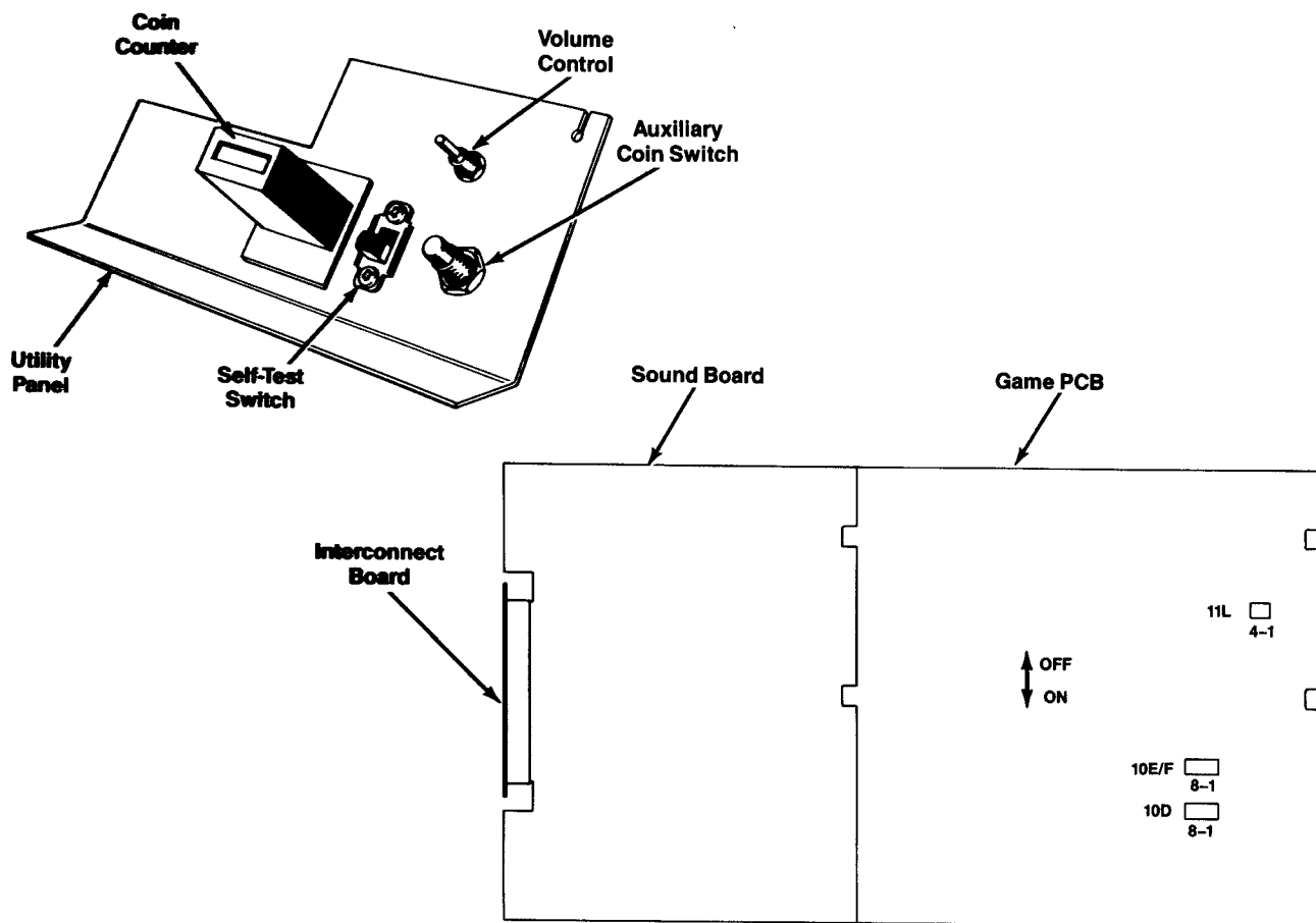
Figure 1-3 Switch Locations
