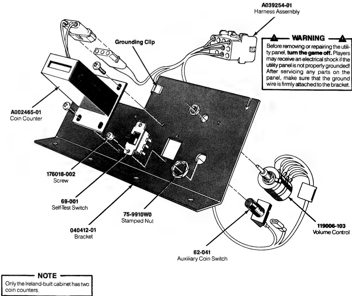
Figure 5-5 Utility Panel Assembly US-Built Cabinet A040413-01 B Ireland-Built Cabinet A040413-02 B Parts List
