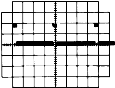
Figure 3 VECTOR (Short) at VECTOR Test Point
