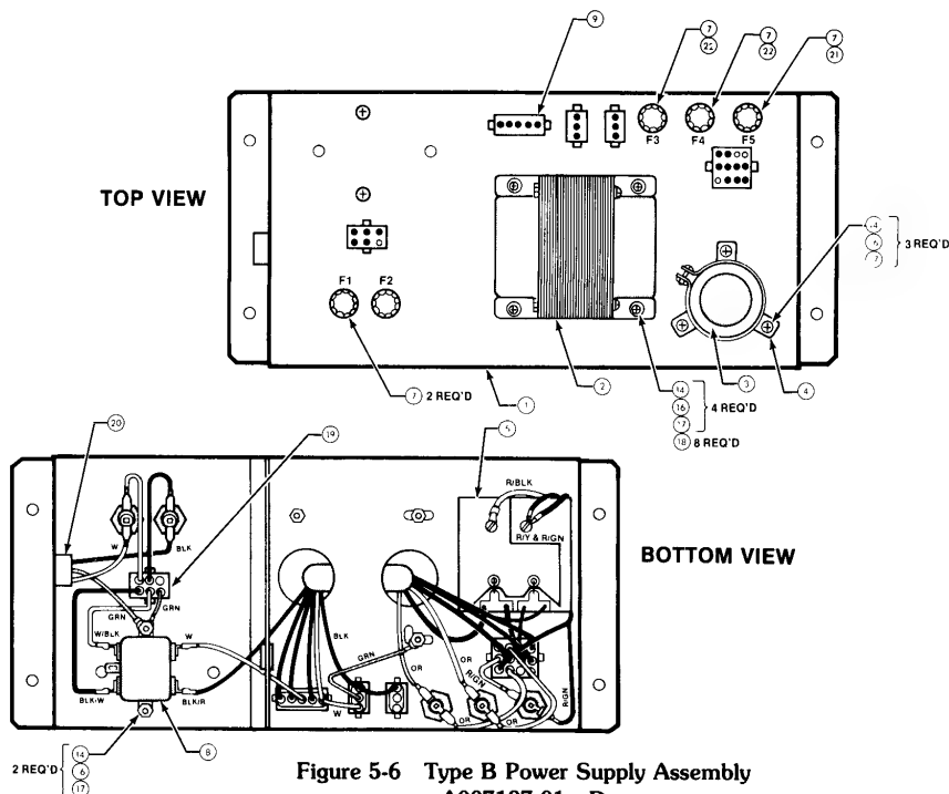
Figure 5-6 Type B Power Supply Assembly Parts List
