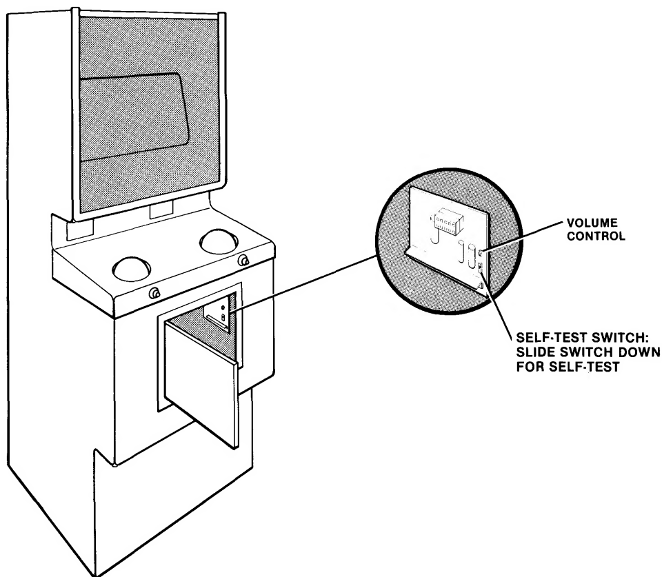
Figure 1-4 Volume Control and Self-Test Switch
