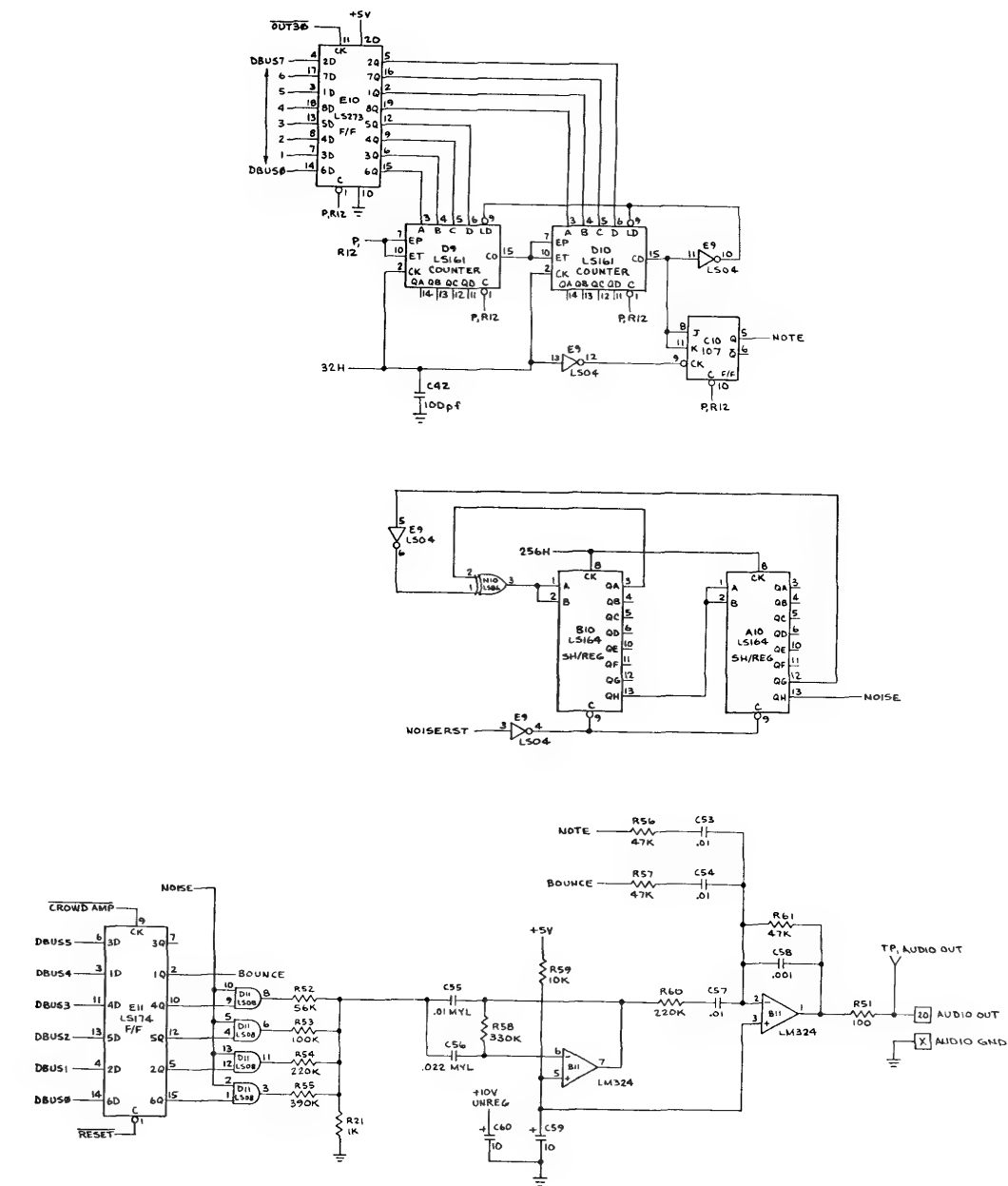
Figure 4-14 Audio Schematic Diagram (Part of Game PCB 034268-XX A)
