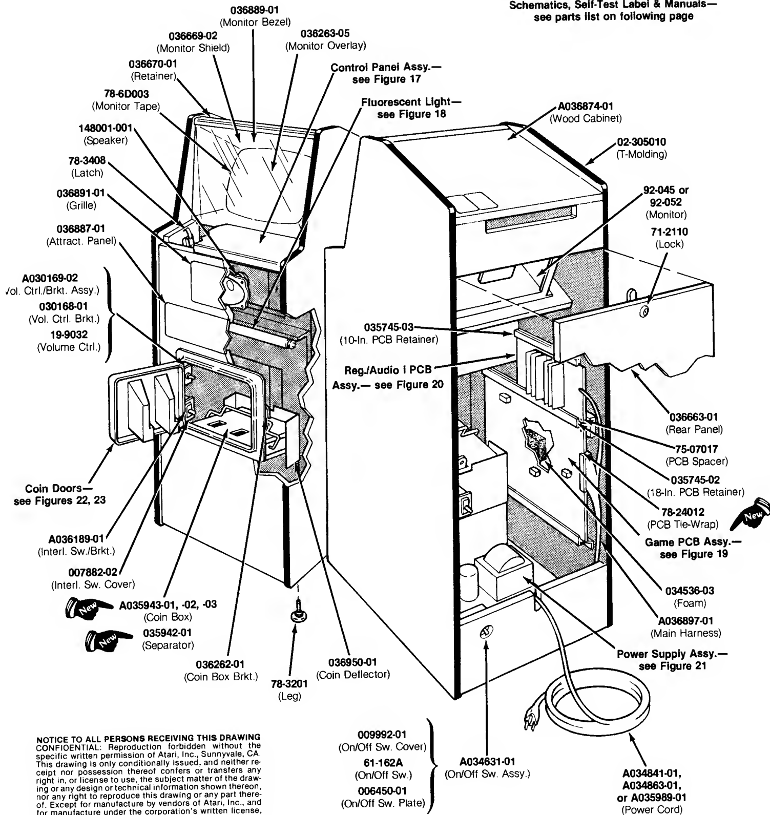
Figure 16 Cabinet-Mounted Assemblies A036873-xx A
