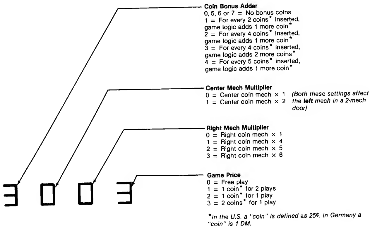
Figure 6 Self-Test Procedure, continued
