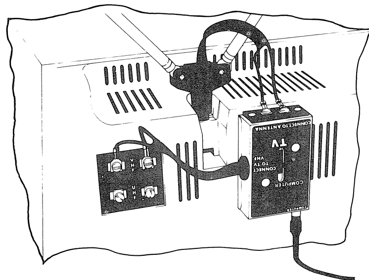
Figure 1. Mounting Switchbox onto TV Set (Connections may vary, depending on your antenna installation).
