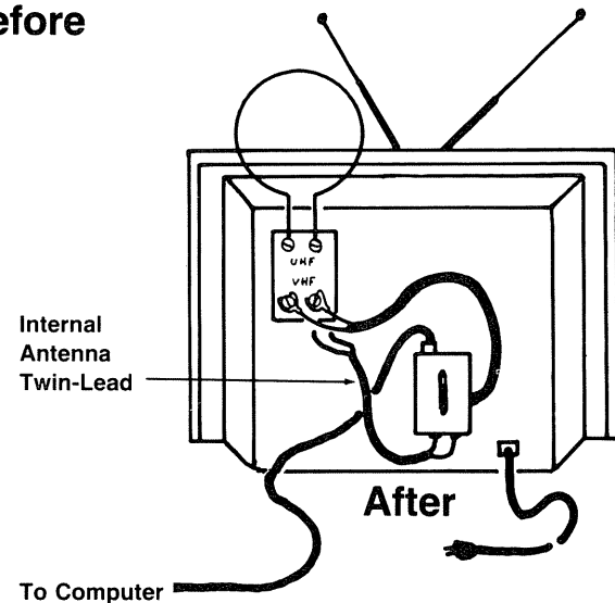
Figure 2. Rear View of TV with Screw Terminals and Internal Antenna.
