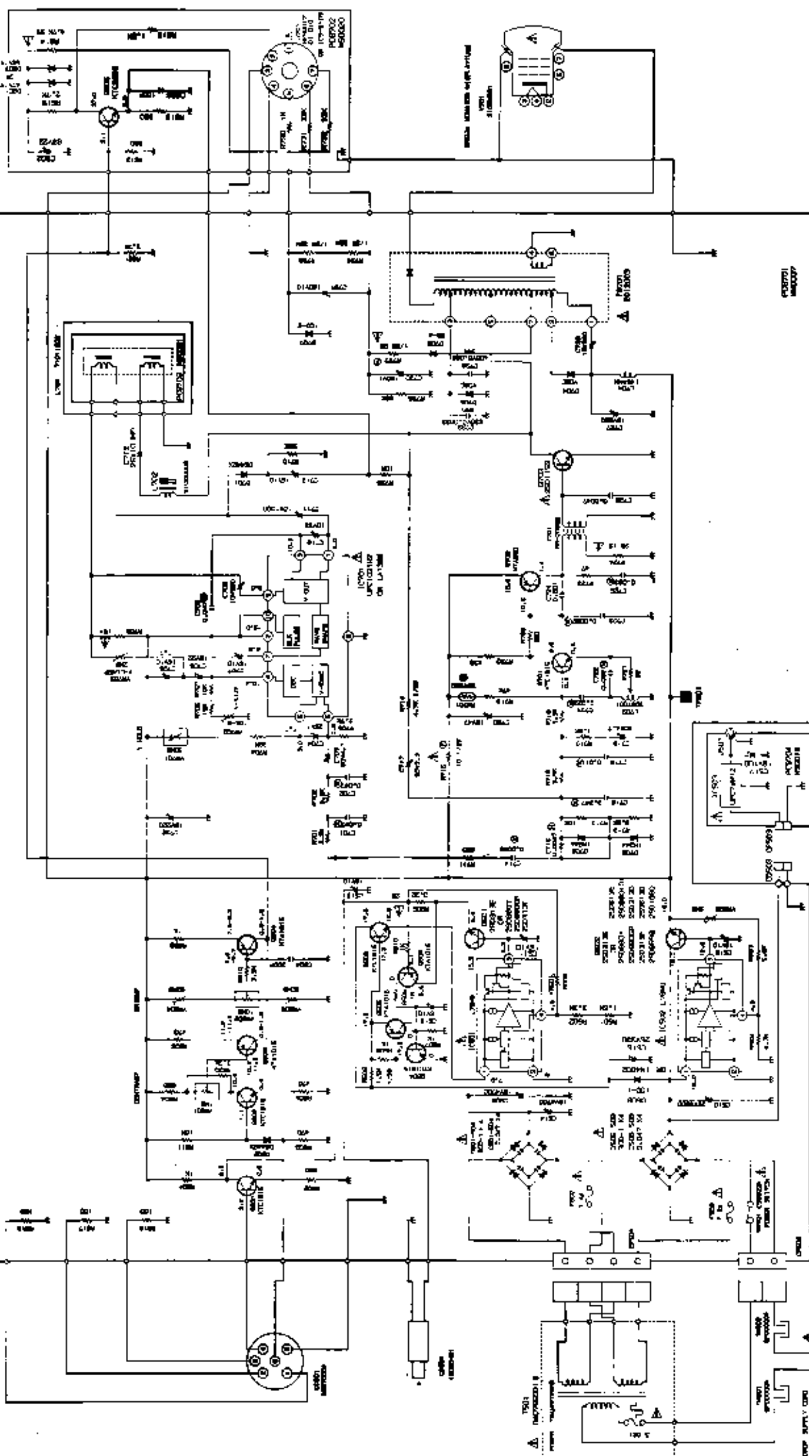
CHASSIS SCHEMATIC DIAGRAM
