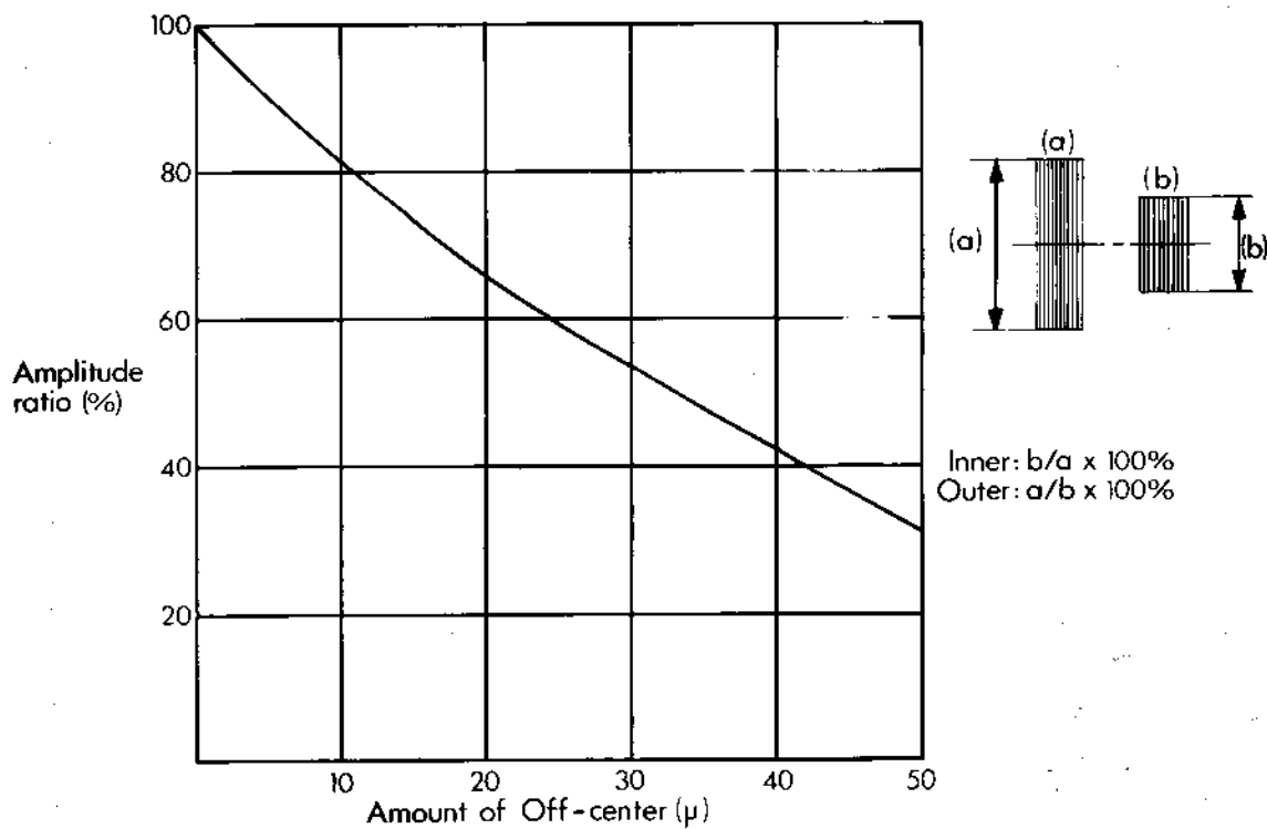
Fig. 5-2 Off-centre calibration curve (Effective width of read head is 180μ)
