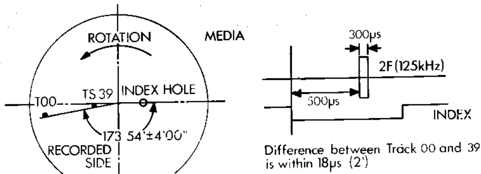
Fig. 2 Waveform of T39 (Index pattern - Radial alignment)
