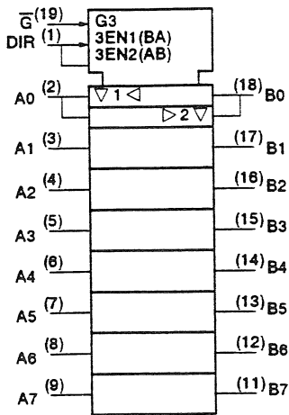
■ Logical Operation Circuit
